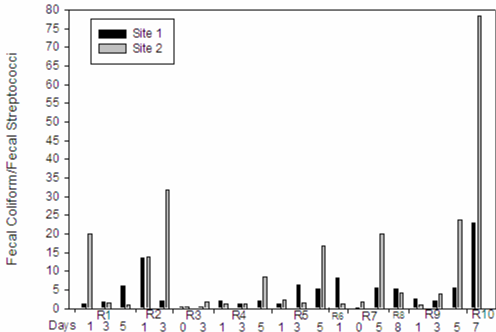
Figure 3-8. Ratio of Fecal Coliform to Fecal Streptococci
