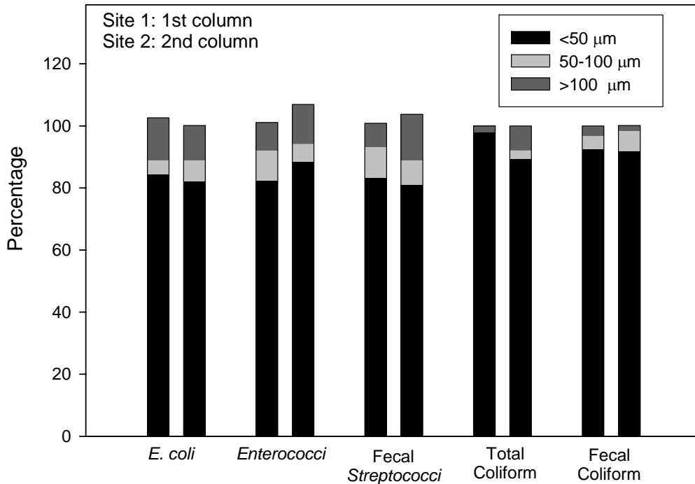
Figure 3-4. Bacteria Distribution in the Sump Water
