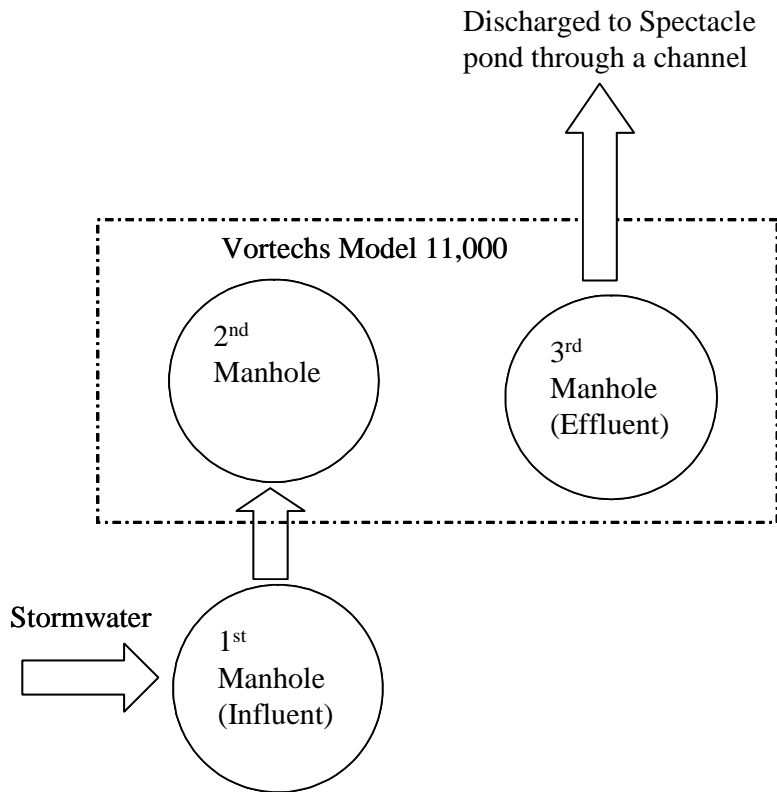
Figure 2-3. Location and Schematics of Sampling Site 2.
