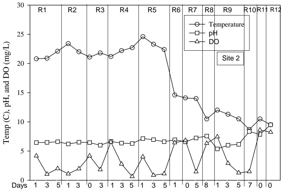
Figure 3-1. Temperature, pH, and DO in the Sump Water
