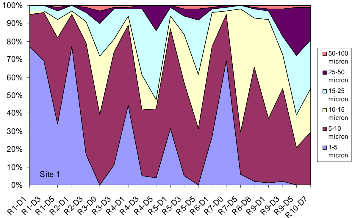
Figure 3-2a. Particle Size Distribution in the Sump Water (Site 1)
