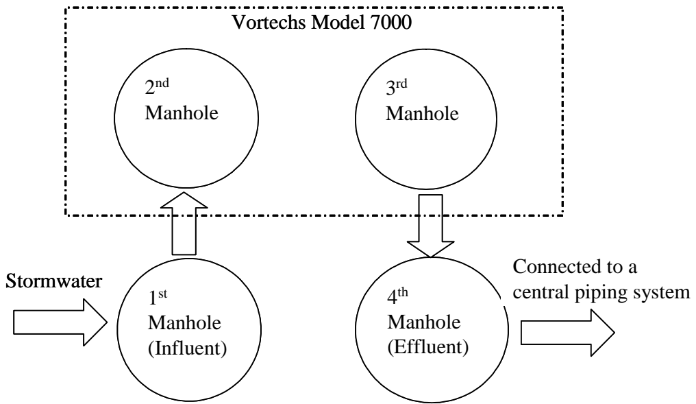
Figure 2-2. Location and Schematics of Sampling Site 1
