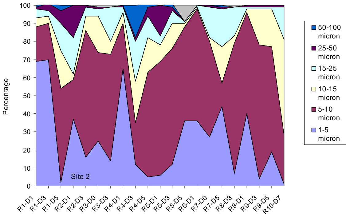
Figure 3-2b. Particle Size Distribution in the Sump Water (Site 2)
